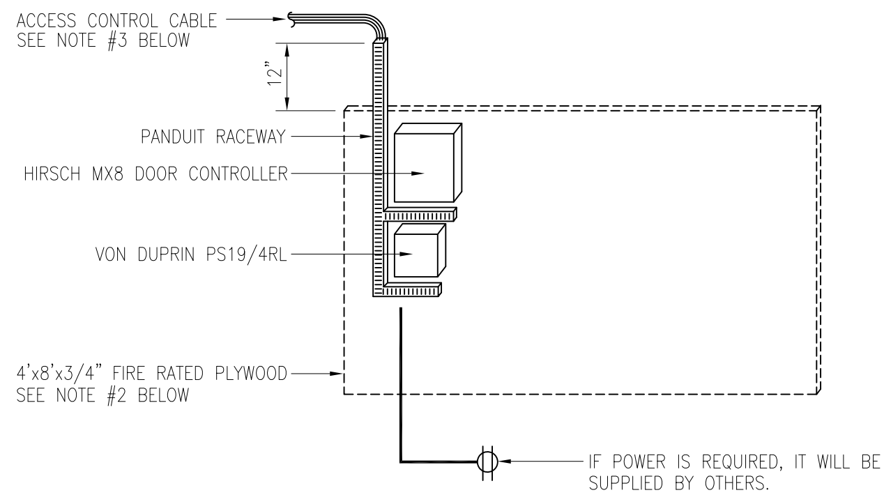
A TYP. (8) CARD READER CONTROL PANEL ASSEMBLY NTS ALL NECESSARY TERMINATIONS BY THIS CONTRACTOR
