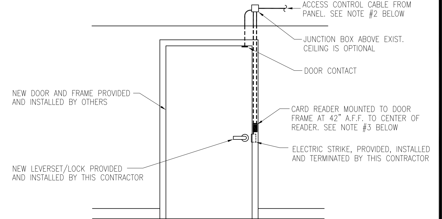
C TYP. NEW SINGLE DOOR CARD ACCESS ASSEMBLY NTS ALL NECESSARY TERMINATIONS BY THIS CONTRACTOR
