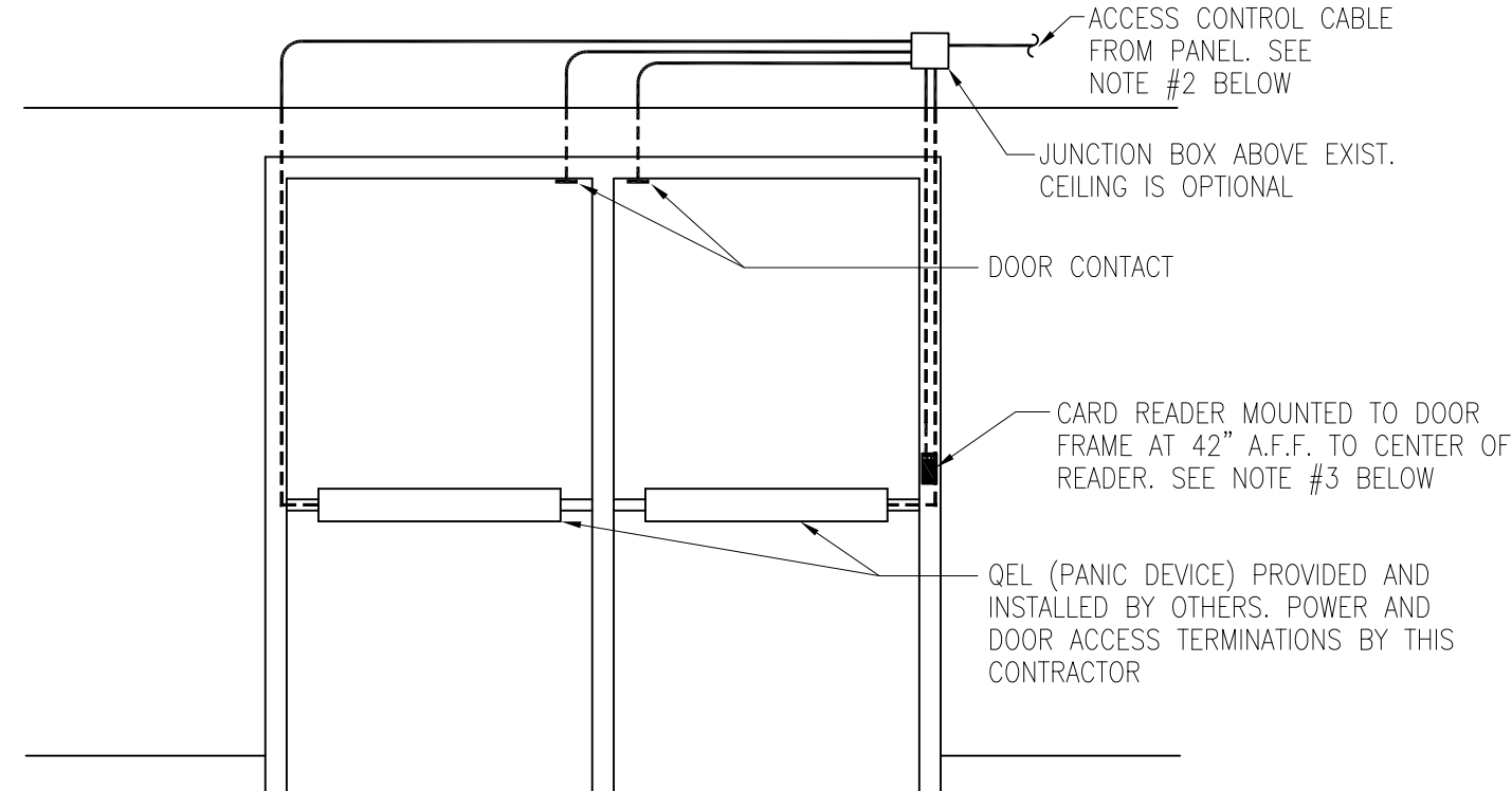
E TYP. DOUBLE QEL DOOR ACCESS ASSEMBLY NTS ALL NECESSARY TERMINATIONS BY THIS CONTRACTOR
