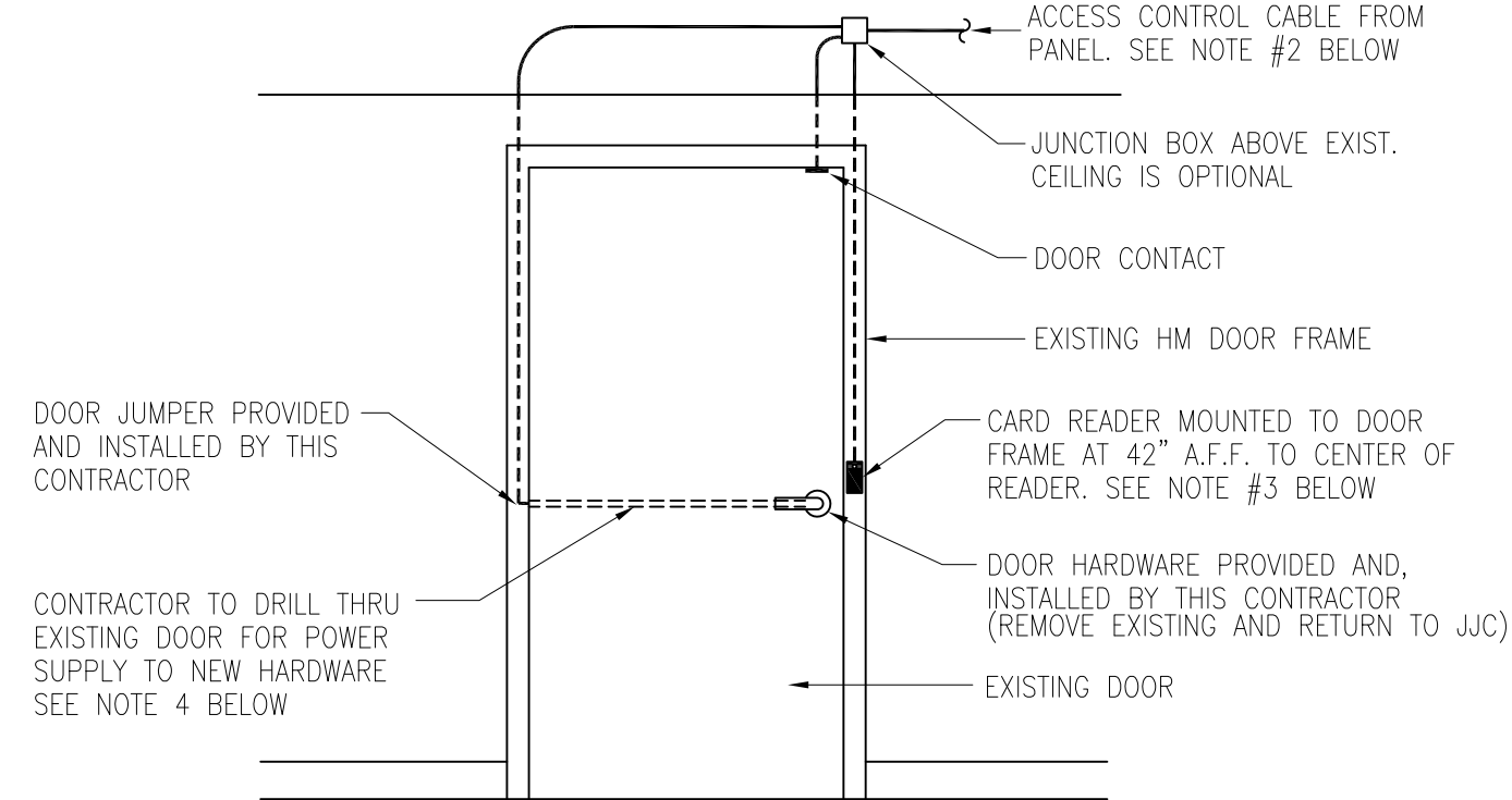
B TYP. EXISTING SINGLE DOOR CARD ACCESS ASSEMBLY NTS ALL NECESSARY TERMINATIONS BY THIS CONTRACTOR
