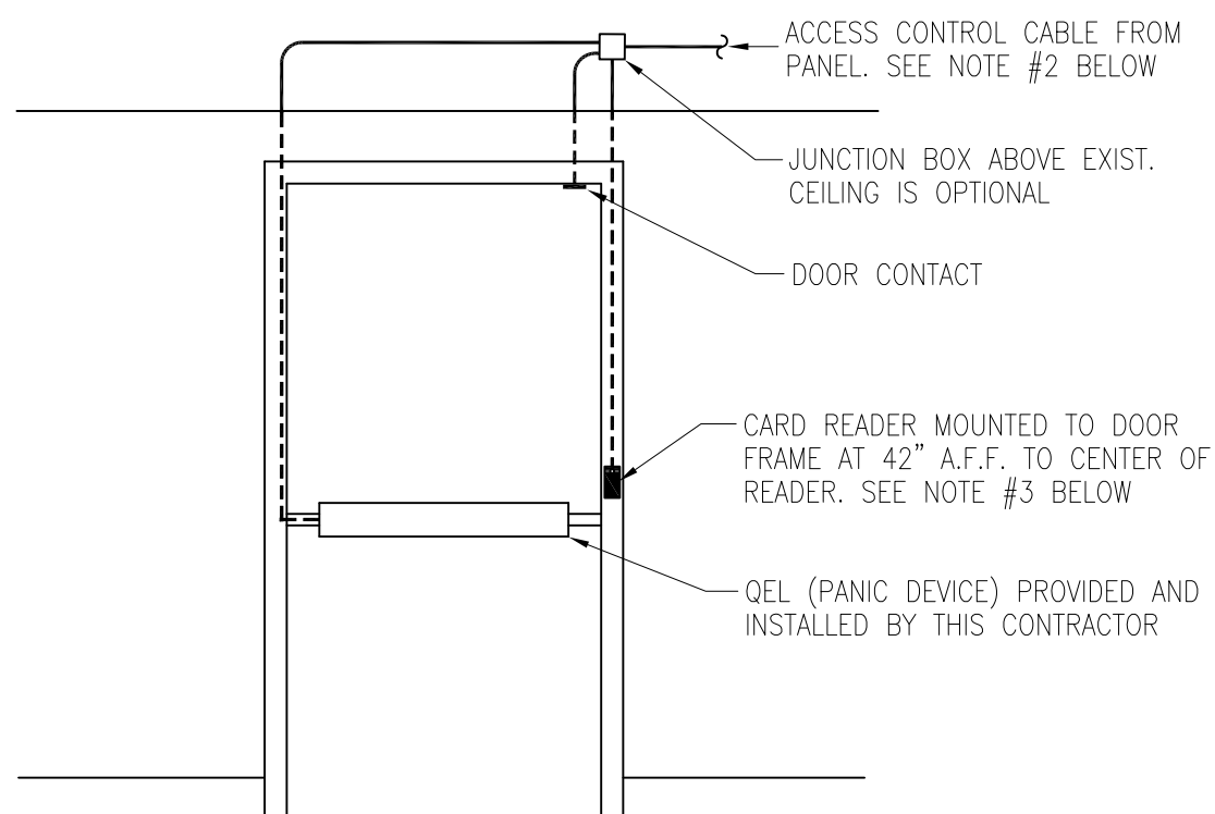
D TYP. SINGLE QEL DOOR ACCESS ASSEMBLY NTS ALL NECESSARY TERMINATIONS BY THIS CONTRACTOR
